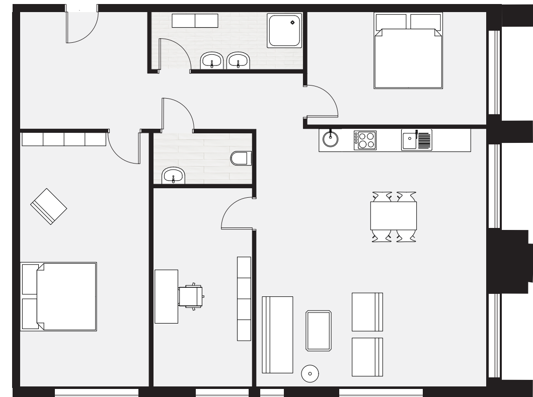
Floorplan 120 m2 apartment 1:100
